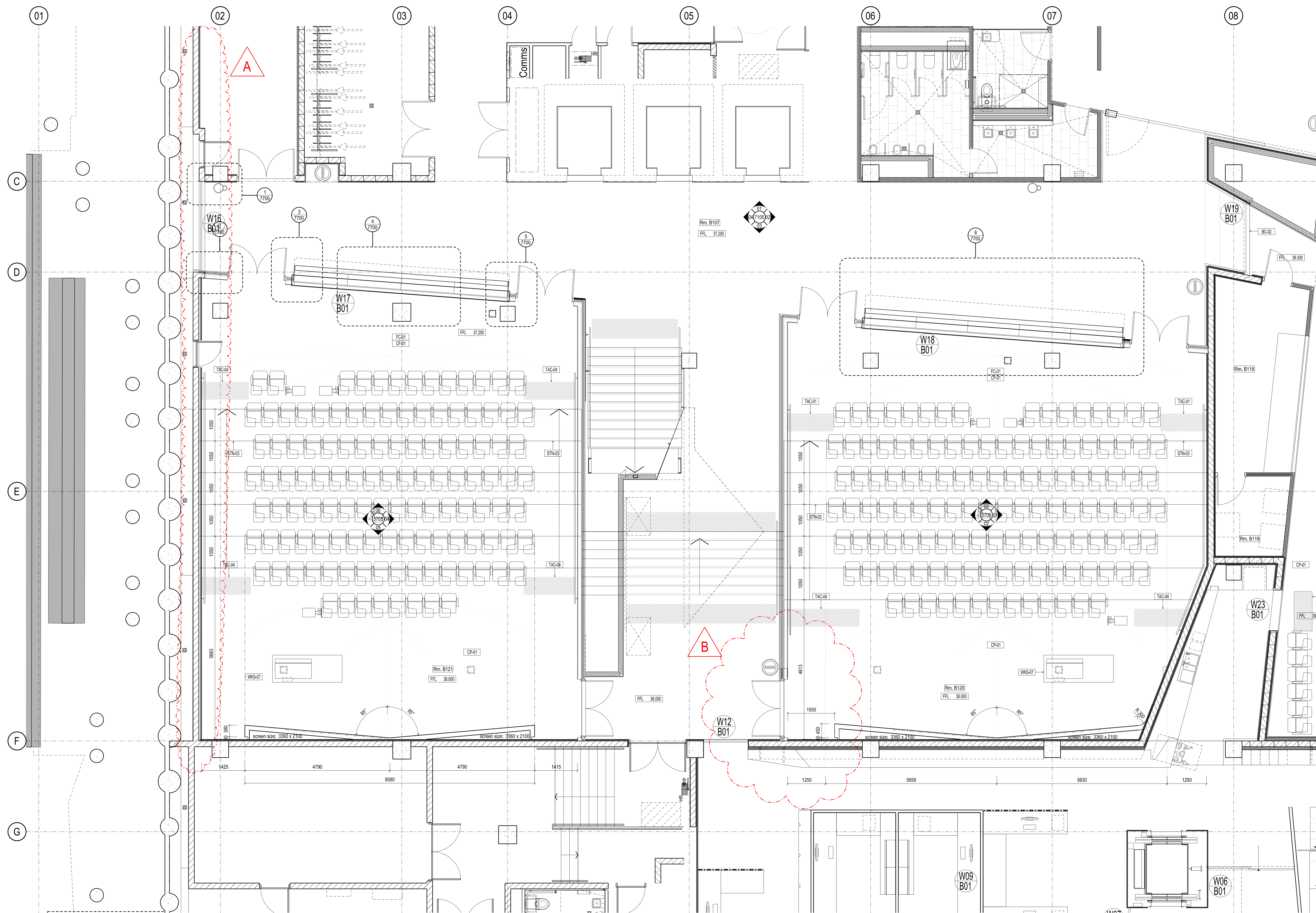
AUDITORIUM 01 & 02 FLOOR PLAN SCALE 1:50
